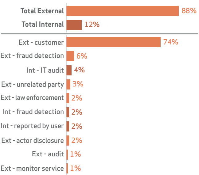
Figure 27. Top 10 discovery methods for financially motivated incidents within Web App Attacks (n=122)
