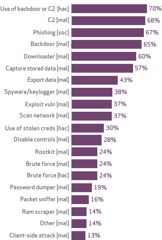
Figure 60. Top threat action varieties within Cyber-espionage (n=426)
