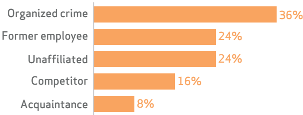
Figure 33. Variety of external actors within Insider Misuse (n=25)
