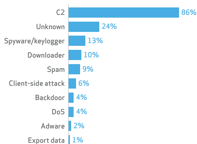
Figure 47. Top 10 threat action varieties within Crimeware (n=2,274)
