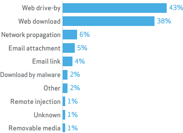
Figure 48. Top 10 vectors for malware actions within Crimeware (n=337)
