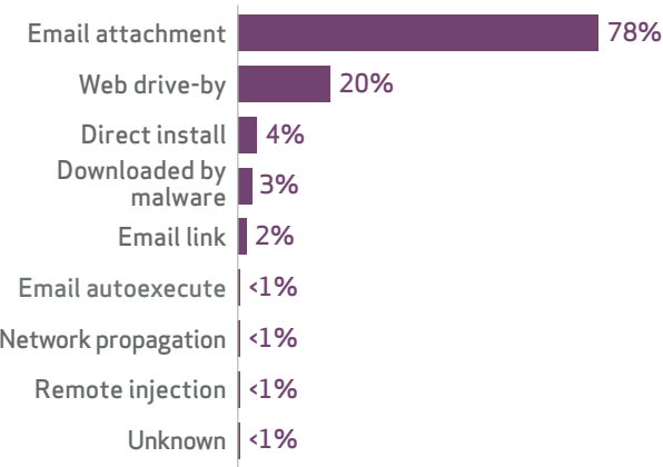
Figure 61. Vector for malware actions within Cyber-espionage (n=329)
