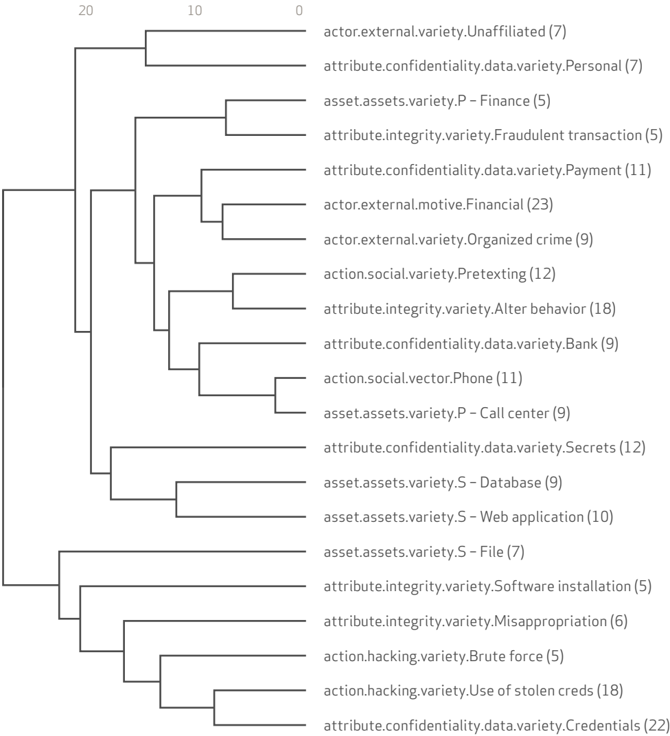
Figure 66. Hierarchical clustering of VERIS enumerations for confirmed data disclosures falling outside the main incident patterns
